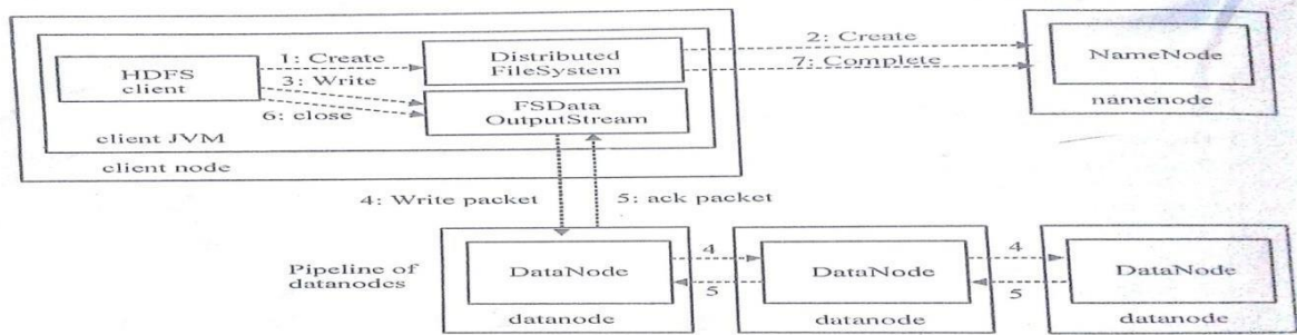
Figure 4.16: Writing data from HDFS
