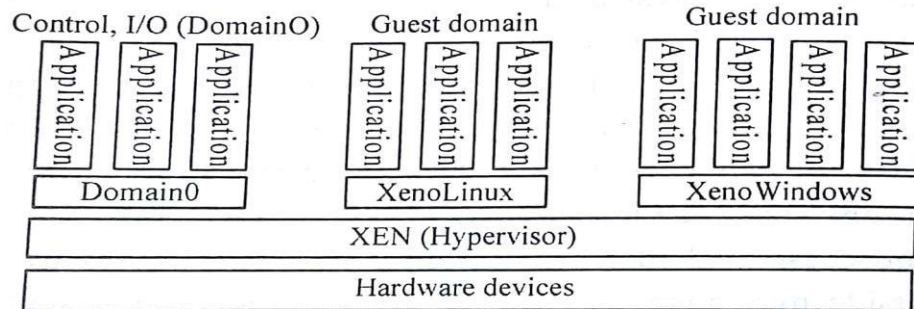
Figure 3.19: Xen architecture’s special domain 0 for control and I/O, and several guest domains
