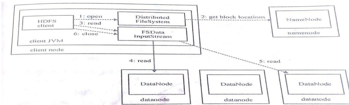
Figure 4.15: Reading data from HDFS
