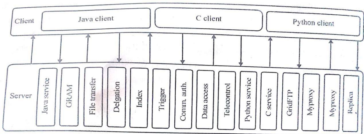
Figure 4.7: Client and GT4 server interactions (vertical boxes correspond to service programs and horizontal boxes represent the user codes)
