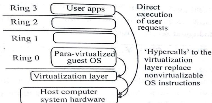
Figure 3.22: Use of a para-virtualized guest OS assisted by intelligent compiler
