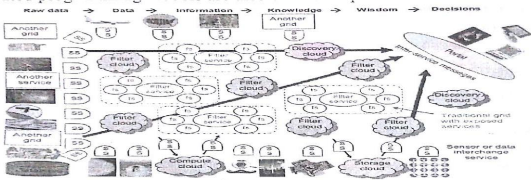
Figure 1.20: The evolution of SOA: grids of clouds and grids, where “SS” refers to a sensor service and “fs” to a filter or transforming service
