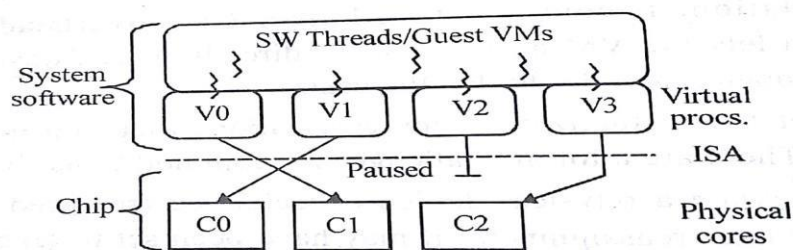
Figure 3.26: Multicore virtualization method exposes four VCPUs to software, when only three cores
