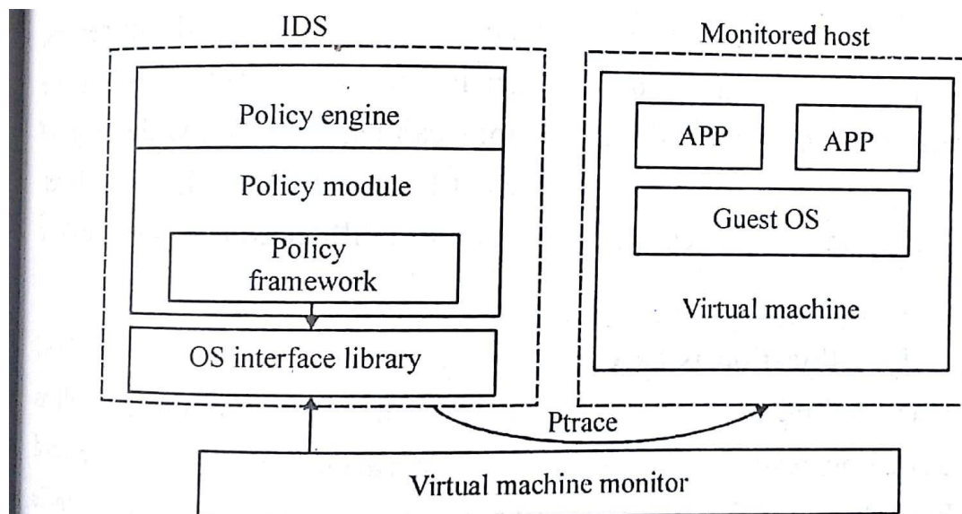
Figure 3.35: Architecture of livewire for intrusion detection using a dedicated VM
