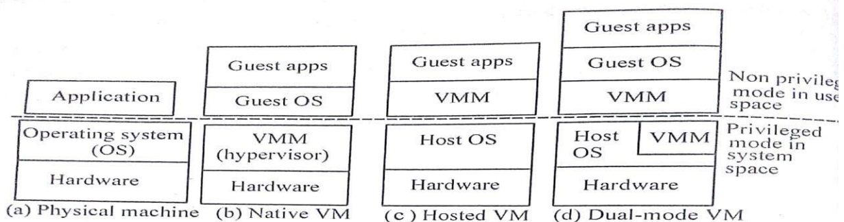
Figure 1.12: Three VM architectures in (b), (c), and (d), compared with the traditional physical machine shown in (a)
