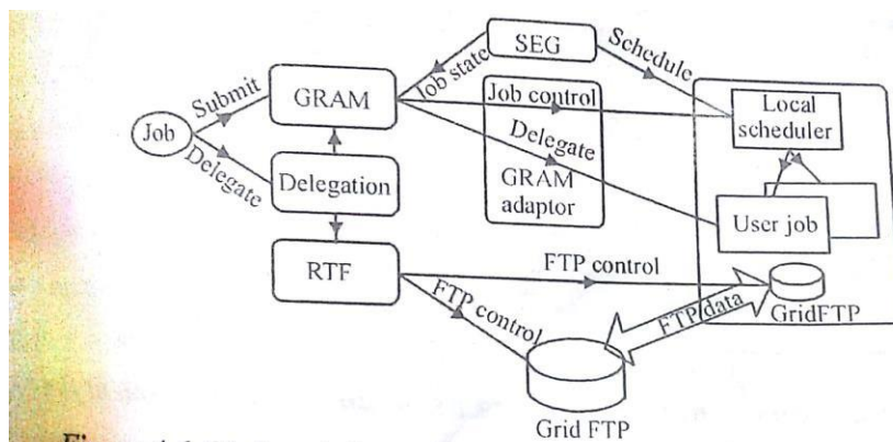
Figure 4.6 Globus job workflow among interactive functional modules
