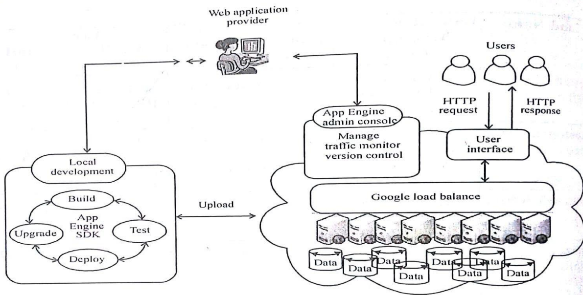
Figure 3.11: Google App Engine platform for PaaS operations
