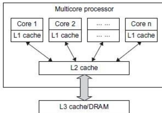
FIGURE 1.5 Schematic of a modern multicore CPU chip using a hierarchy of caches, where L1 cache is private to each core, on-chip L2 cache is shared and L3 cache or DRAM is off the chip.
