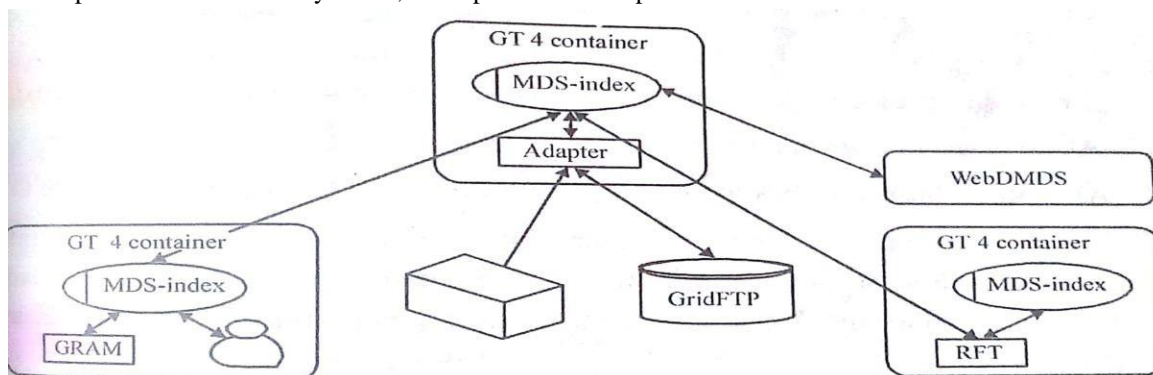
Figure 4.9: GT4 system monitoring and resource discovery infrastructure
