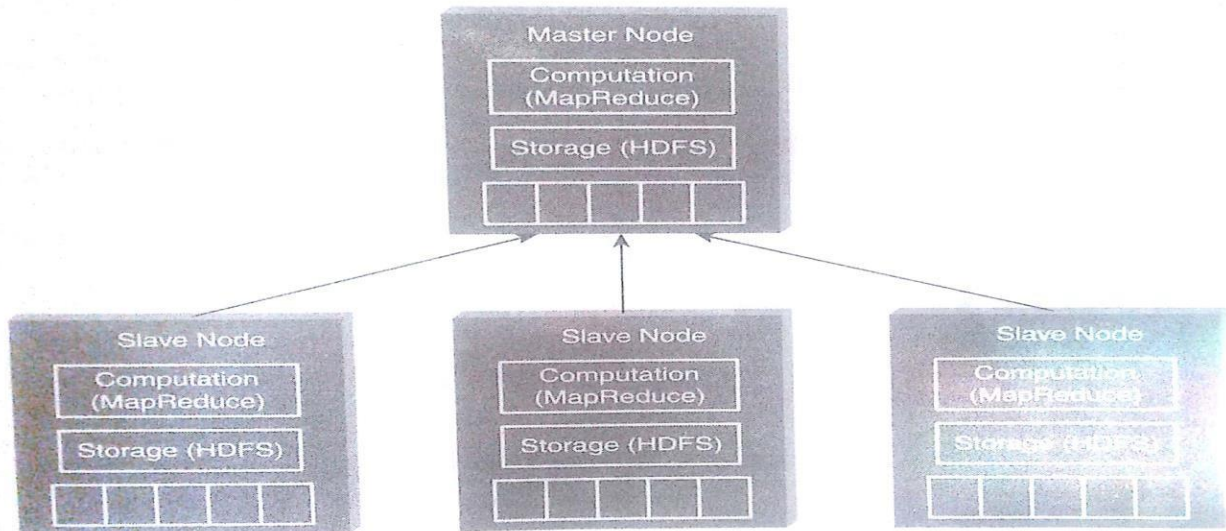
Figure 5.10 Hadoop high-level architecture. Reference: Hadoop in Practice, Alex Holmes.
