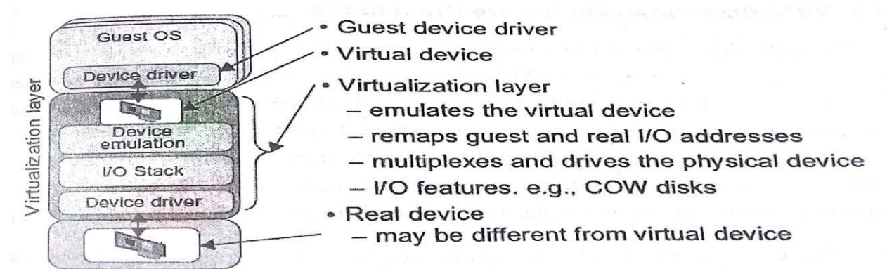
Figure 3.25: Device emulation for I/O virtualization
