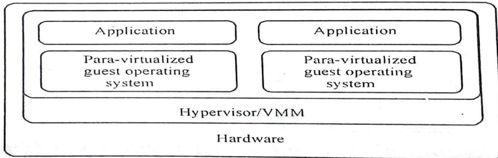
Figure 3.21: Para-virtualized VM architecture
