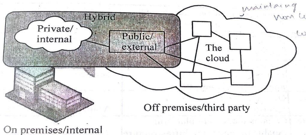
Figure 3.4: Hybrid cloud
