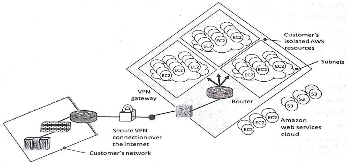
Figure 3.9: Amazon VPC
