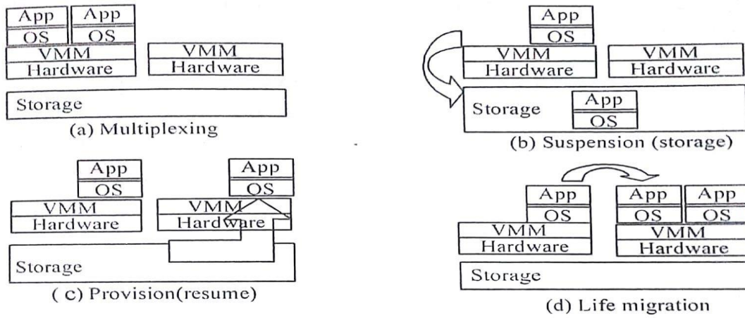
Figure 1.13: VM multiplexing, suspension, provision and migration in a distributed computing environment.
