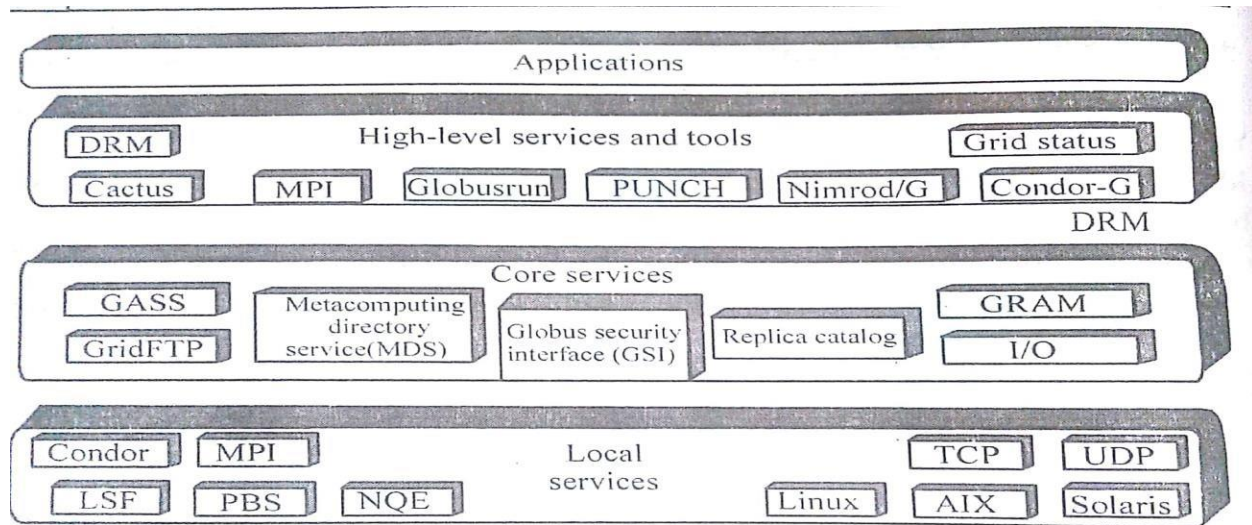
Figure 4.4: Globus Toolkit GT4 supports distributed and cluster computing services
