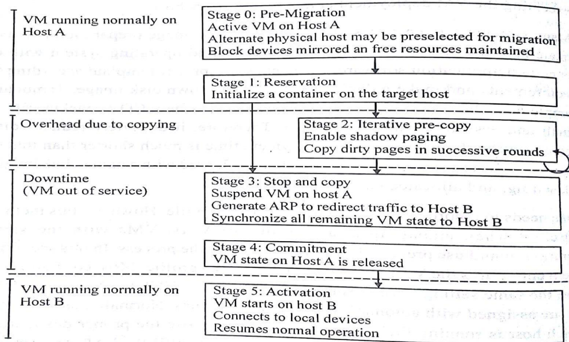
Figure 3.31: Live migration process of a VM from one host to another
