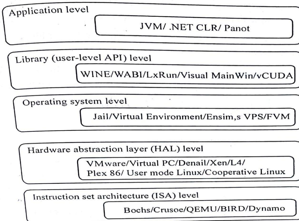
Figure 3.14: Virtualization: From hardware to applications - five abstraction levels
