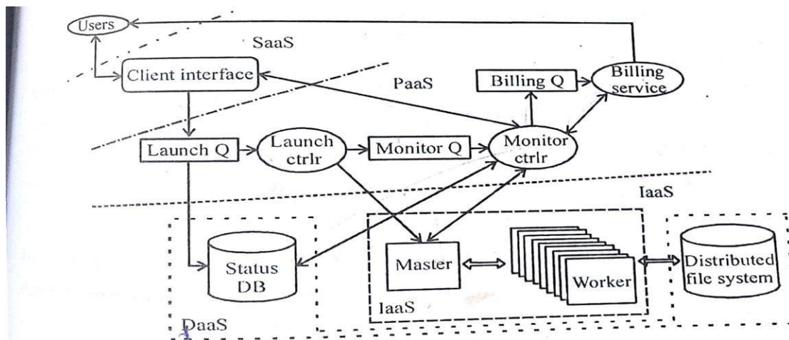
Figure 3.7: IaaS, PaaS, and SaaS cloud service models at different service levels
