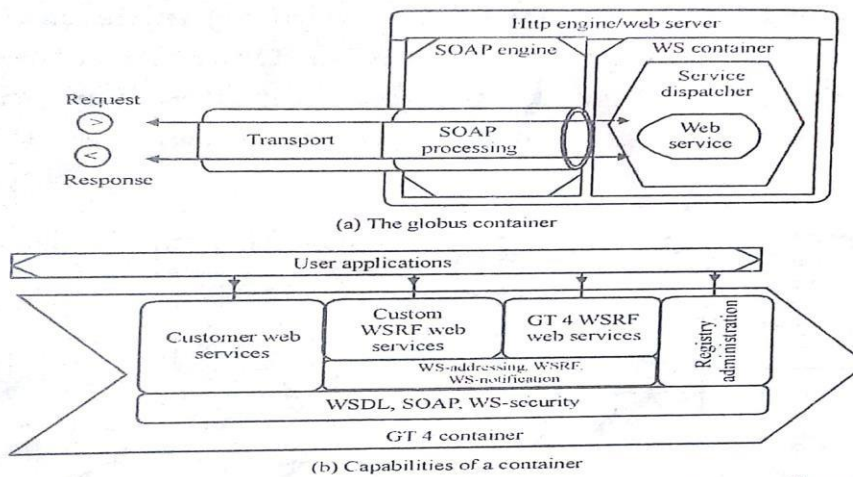
Figure 4.8: Globus container serving as a runtime environment for implementing web services
