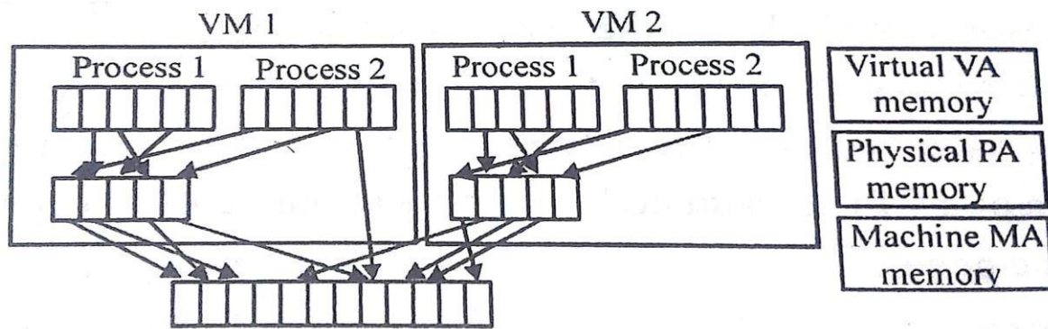
Figure 3.24: Two-level memory mapping procedure
