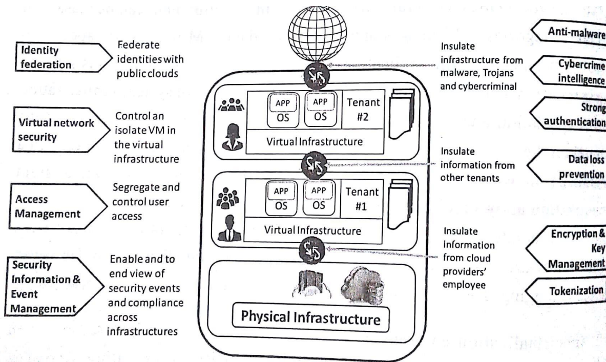
Figure 3.36: Techniques for establishing trusted zones for virtual cluster insulation and VM isolation
