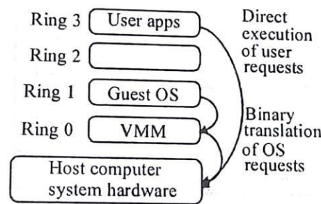
Figure 3.20: Indirect execution of complex instructions via binary translation of guest OS requests
